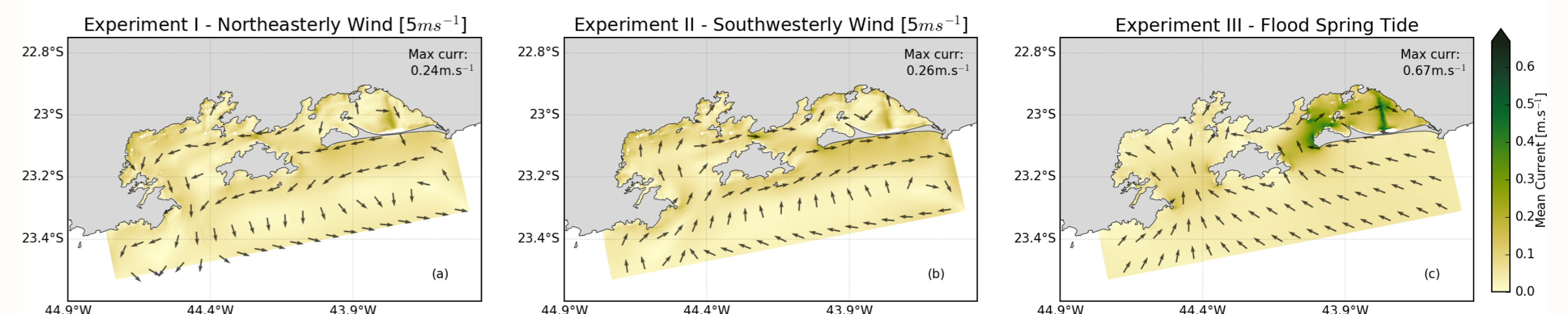
Figure 3 : Mean current no Experiments I, II and III. Panels (a) and (b) represent the current in the last instant modelled and panel (c) represent the flooding spring tides.
